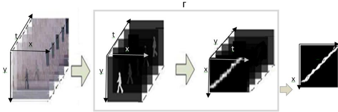
Fig. 2: An xt pattern extraction- Operator \Gamma shows rotating traditional space-time volume and displacing its axes.
