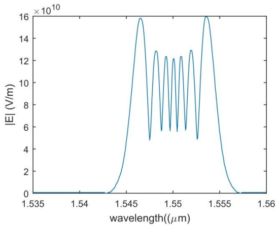
Figure 2: Spectral broadening of the input pulse for \text{MoS}_2 coated Si waveguide with a length of 3mm.
