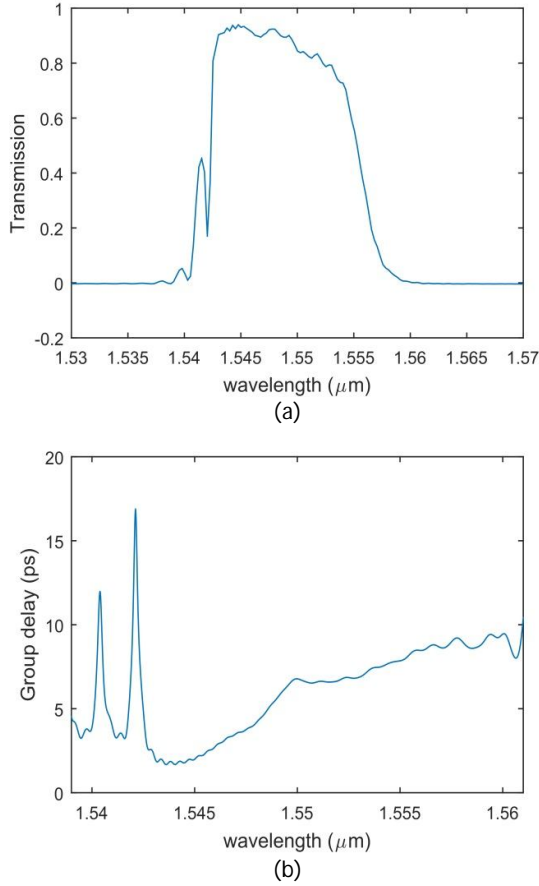
Figure 4: (a) Transmission and (b) group delay of the chirped Bragg grating versus wavelength.
