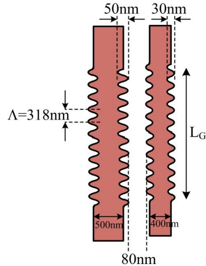
Figure 3: The Bragg grating and its structural parameters.
