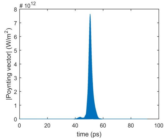
Figure 5: Output pulse versus time for the first pulse compressor design. FWHM of this pulse is approximately 2ps implying a compression ratio of 2.5.
