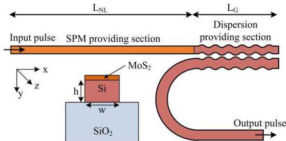
Figure 1: Top view of the proposed pulse compressor along with the device cross section.
