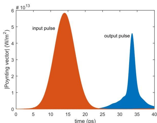
Figure 6: The input and compressed output pulses for the second design.
