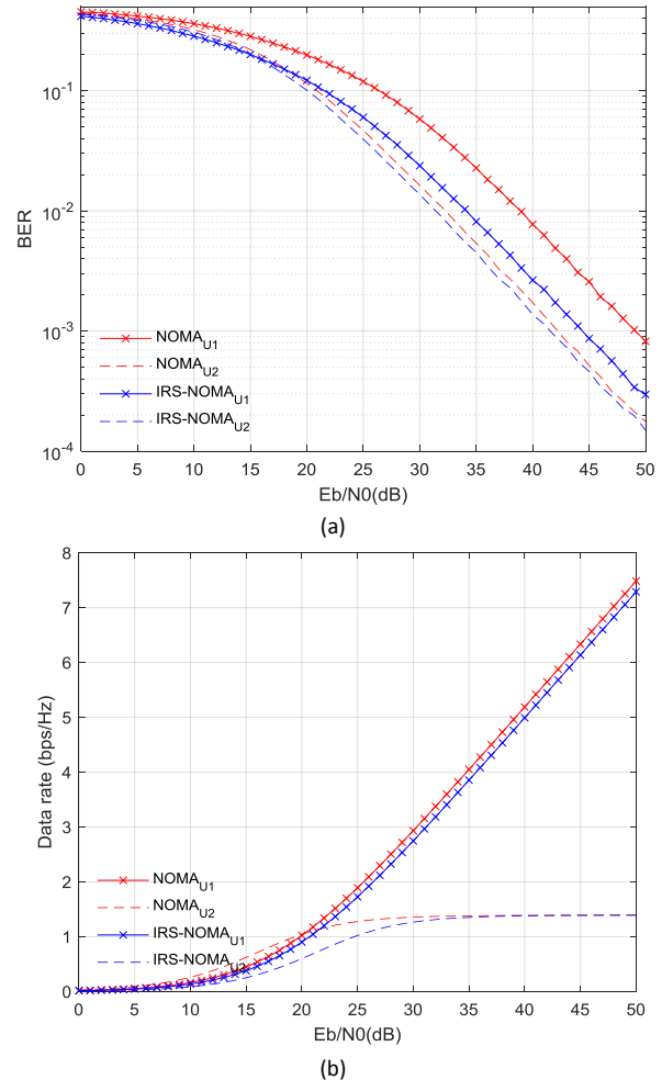
Fig. 2: Comparison of user performance in the NOMA and IRS-NOMA systems in terms of (a) BER and (b) data rate.
