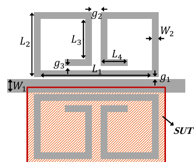
Fig. 1: Proposed microwave moisture sensor.
