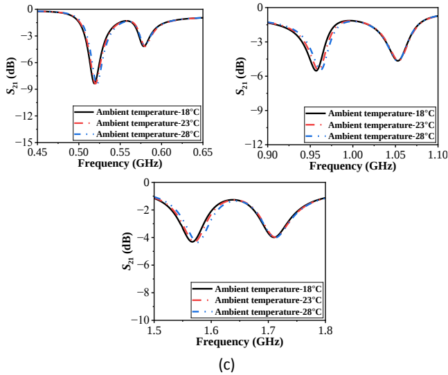
Fig. 10: Simulation results of ambient temperature variation for wheat grains at different MCs: (a) 10%, (b) 20%, (c) 30%.
